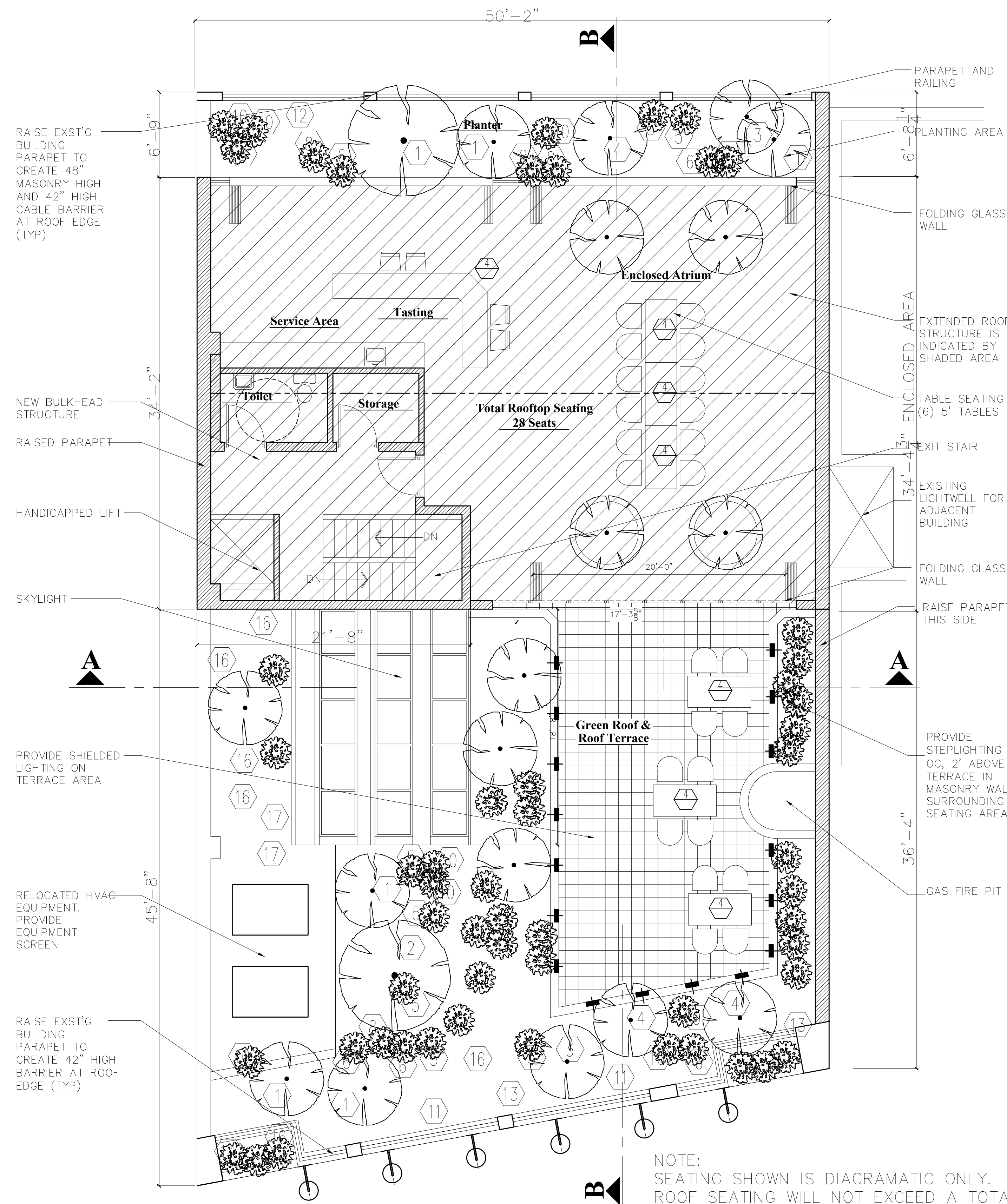
ROOF PLAN (OCCUPIED) SCALE: 3/16"=1'-0"
